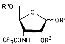
3 R^1 = Me, R^2 = R^5 = Bz 4 R^1 = Me, R^2 = R^5 = p\text{-NO}_2Bz 5 R^1 = R^2 = Ac, R^5 = Bz 6 R^1 = Ac, R^2 = R^5 = Bz 7 R^1 = Ac, R^2 = R^5 = p\text{-NO}_2Bz
